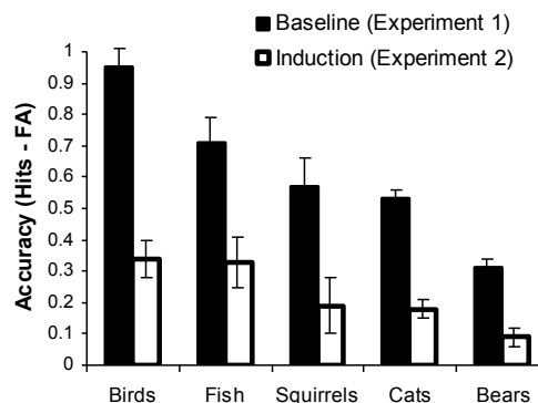
Figure 2: Mean accuracy (Hits – FA) across target categories in Experiment 1 and 2.
